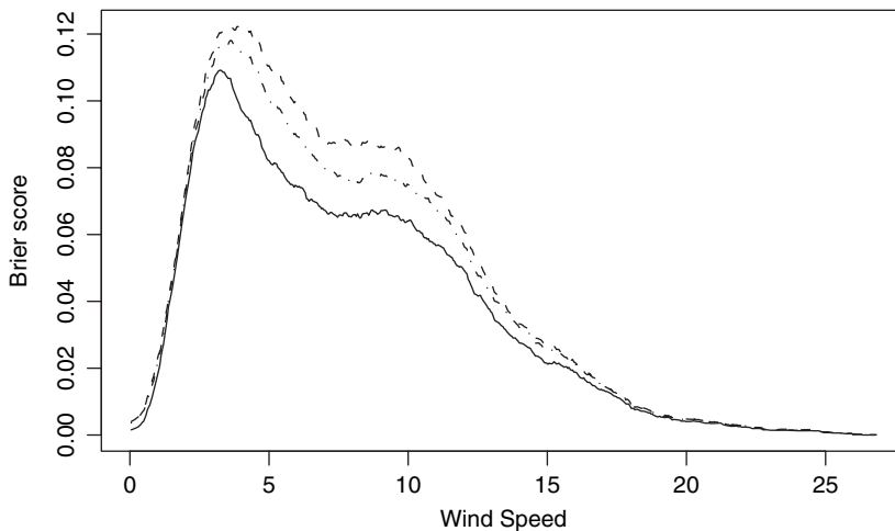
Fig. 10. Brier score plot for persistence forecasts (-----), autoregressive forecast (-.-.-.-) and RST forecasts (—) of hourly average wind speed at the Stateline wind energy centre, in metres per second: the graphs show the Brier score as a function of the threshold value; the area under each forecast's curve equals the CRPS value (14)
