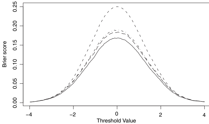
Fig. 3. Brier score plot for the ideal forecaster (—), climatological forecaster (· · · · ·), unfocused forecaster (- · - · -) and Hamill's forecaster (- - -): the curves show the Brier score as a function of the threshold value; the area under each forecaster's curve equals the CRPS value (14)
