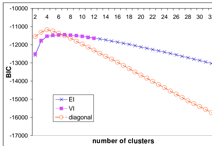
Figure 2: Average BIC values for synthetic data based on the ovary data: Mixture of 4 multivariate normal distributions
