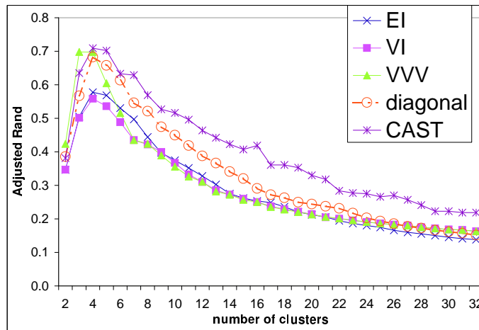
Figure 1: Average adjusted Rand indices for the synthetic data based on the ovary gene expression data: Mixture of 4 multivariate normal distributions
