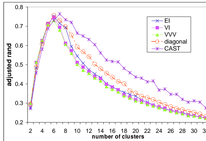
Figure 5: Average adjusted Rand indices for the synthetic cyclic data sets.
