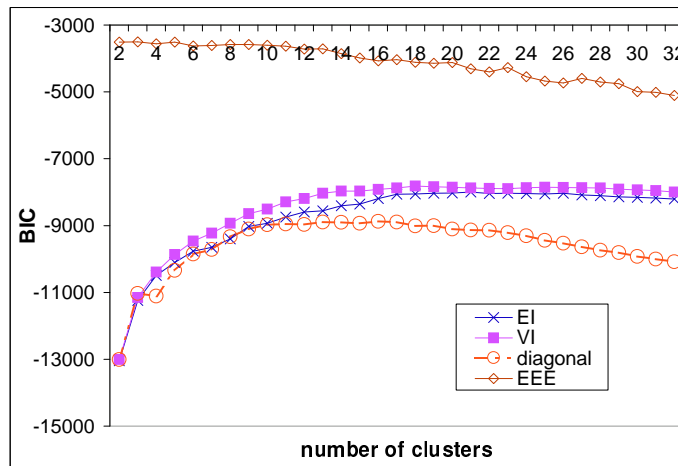
Figure 14: Average BIC values for the log transformed yeast cell cycle data with the 5-phase criterion.
